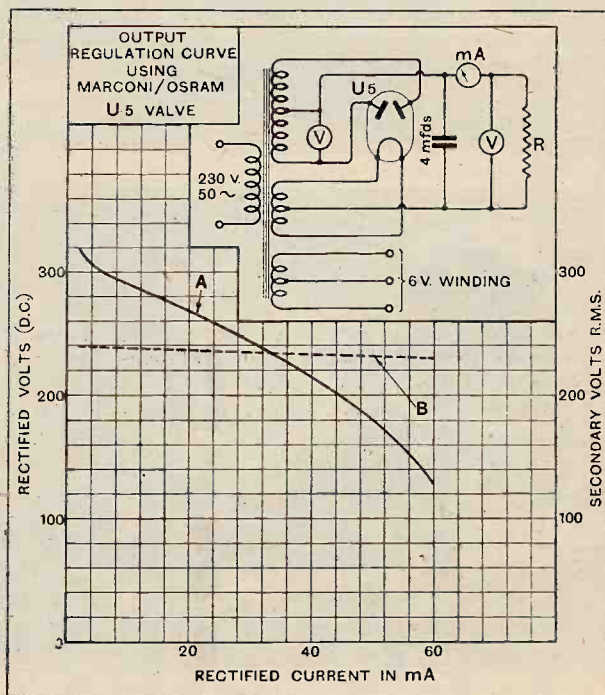
Output voltage regulation curves. The full-line curve A shows the rectified voltage under load while the curve B is the corresponding R.M.S. secondary voltage.
