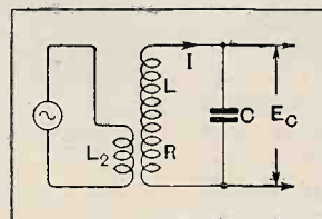
Fig. 1.—Simple series tuned circuit. If a voltage E is induced into the closed circuit LRC the voltage E_C is built up across it at the resonant frequency. \frac{E_C}{E} is the voltage magnification m of the tuned circuit and is equal to \frac{I}{R} \sqrt{\frac{L}{C}} .
