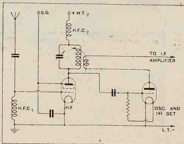
Fig. 1.—Schematic diagram of connections of the first two valves in the Igranic Neutrosonic Short Wave receiver.
