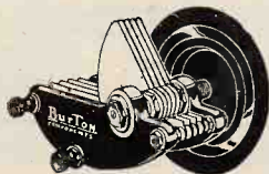
THE BURTON REACTION CONDENSER. Capacity 0001, panel mounting type 4/-
