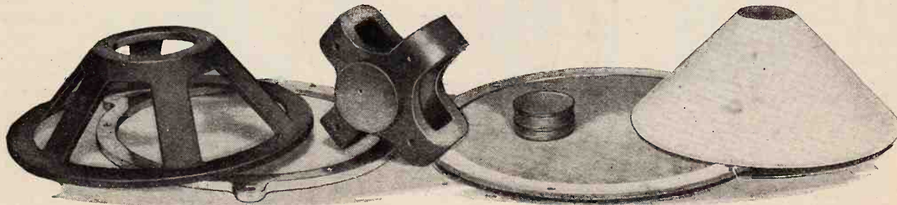
Components used in the construction of the model having the 2 mm. gap. The surround material is secured without stretching to the cardboard rings and the spare material is cut away after the diaphragm has been attached.
