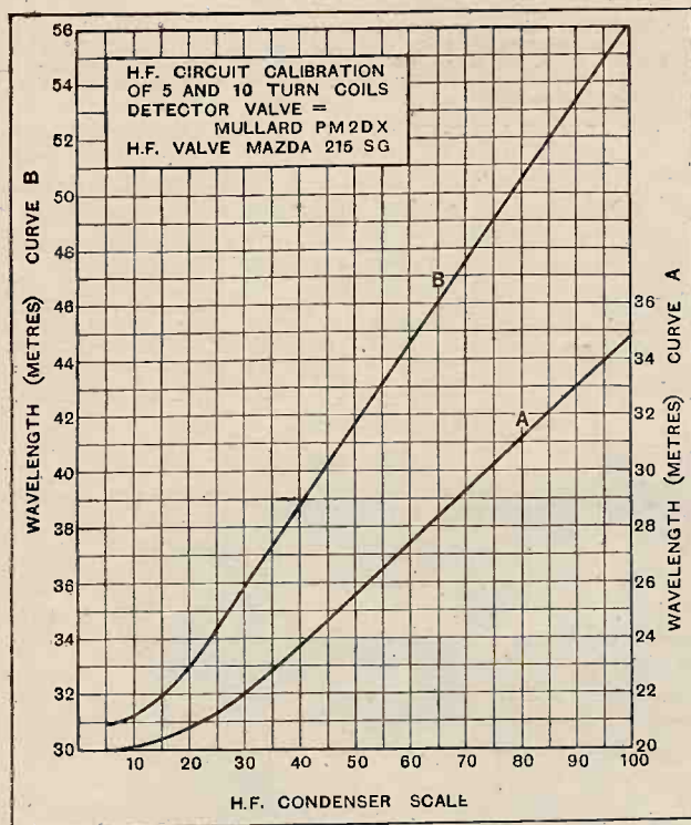
Fig. 8.—Calibration curves of the H.F. coil with reaction adjusted to cause the stage to oscillate weakly.
