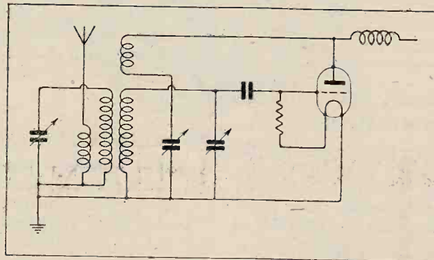
Fig. 1.—A filter circuit preceding a leaky-grid detector.
