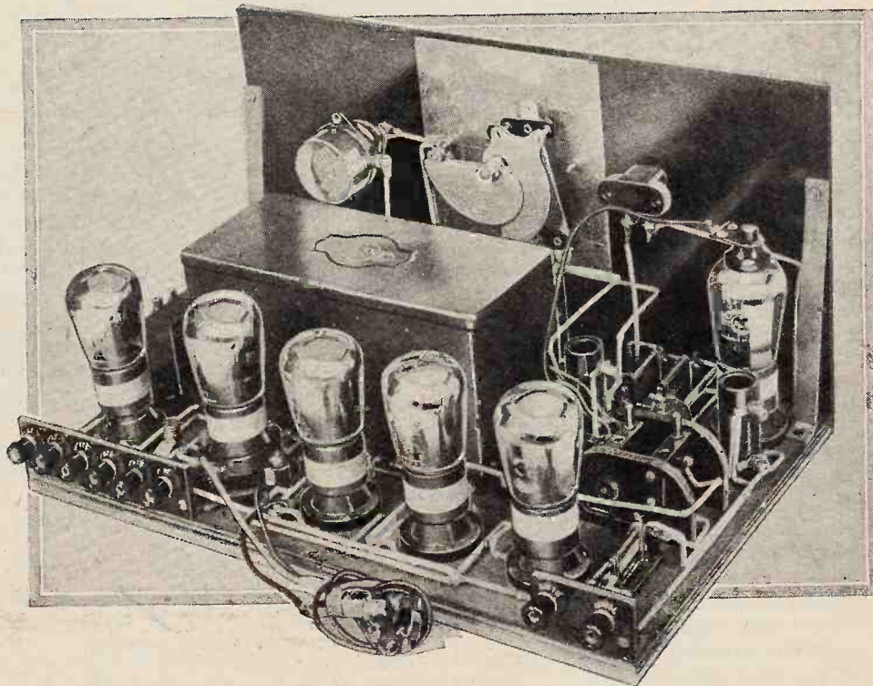
Igranic Neutrosonic Short Wave chassis removed from the cabinet. Note the I.F. amplifier unit and metal screen behind the tuning condenser. The short-wave plug-in coils have been removed to show the H.F. chokes associated with the aerial and screen-grid valve circuits.
