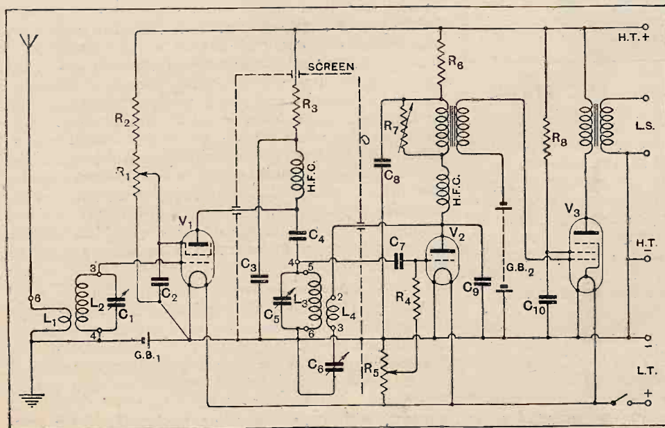
Fig. 1.—The theoretical circuit values are as follows: C_1 and C_5 = 0.00015 mfd., C_2 and C_3 = 0.01 mfd., C_4 and C_6 = 0.0002 mfd., C_7 = 0.0001 mfd., C_8 = 0.000075 mfd., C_9 = 2 mfd., C_{10} = 1 mfd., R_1 = 30,000 ohms, R_2, R_3 and R_6 = 20,000 ohms, R_4 = 5 megohms, R_5 = Polar semi-fixed potentiometer, R_7 = 200,000 ohms, R_8 = 5,000 ohms.
