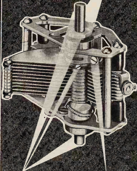
Steel Centre Spindle, adjustable for length and particularly useful for ganging and attaching to Thumb or Drum Control.
