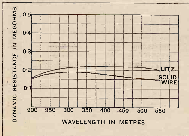
Fig. 4.—Dynamic resistance of tuned circuit with valve and valve-holder in parallel.
